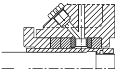
External flushing uncooled stuffing box Stuffing box for external sealing drilled inlet and outlet
